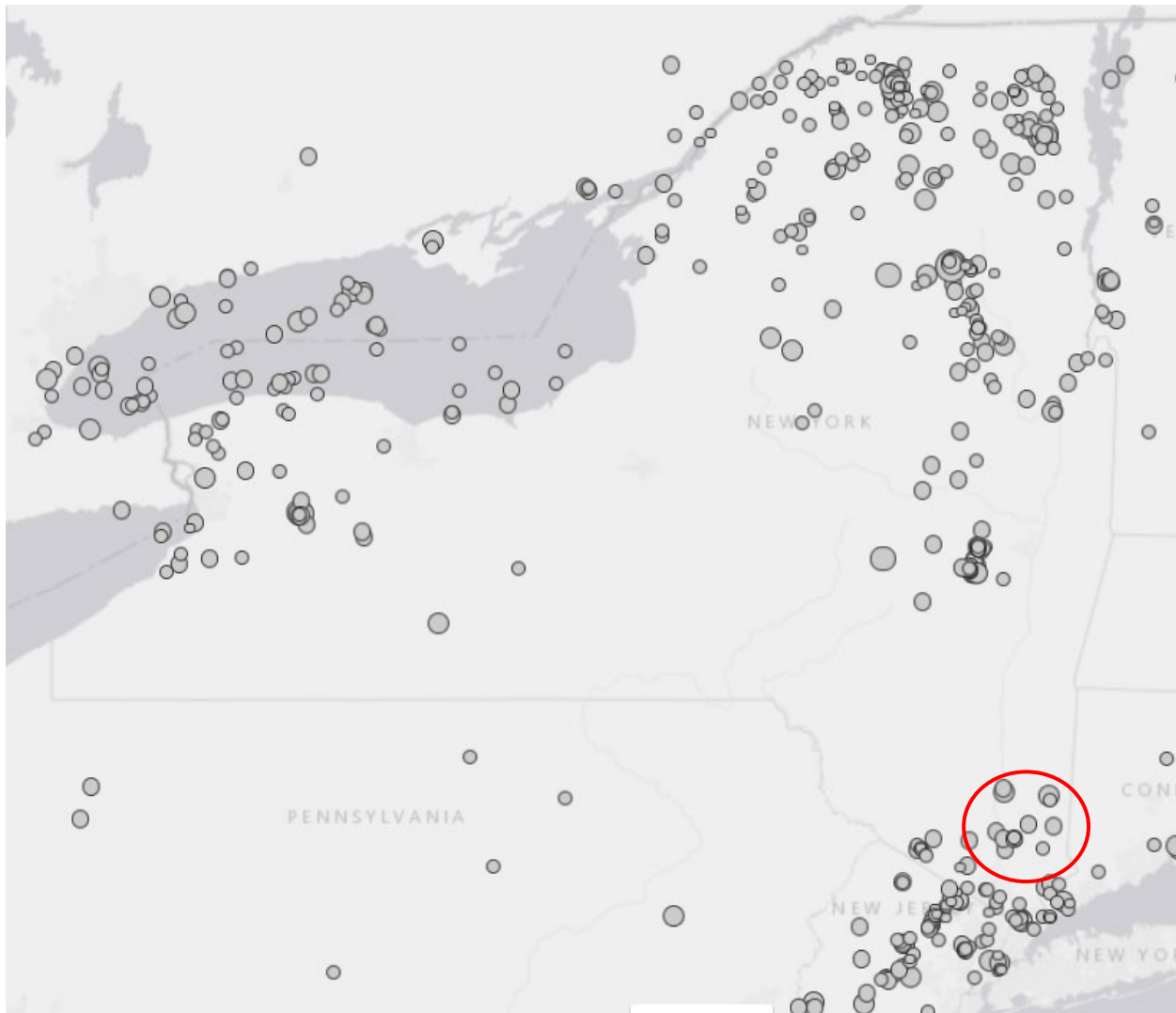
Figure 5.4.3-5. Earthquake Epicenters in the Northeast United States, January 1950 to April 2020
