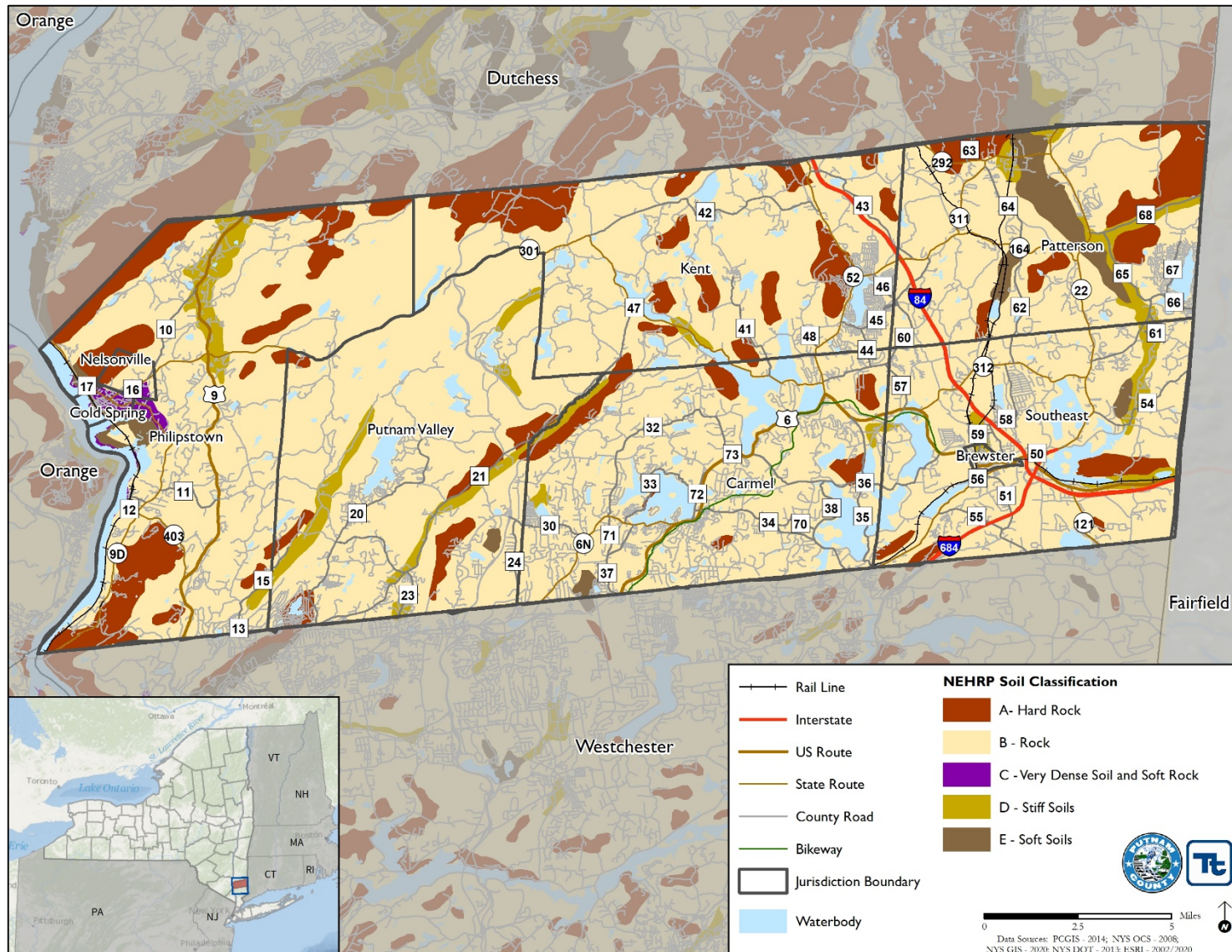
Figure 5.4.3-3. NEHRP Soils in Putnam County
