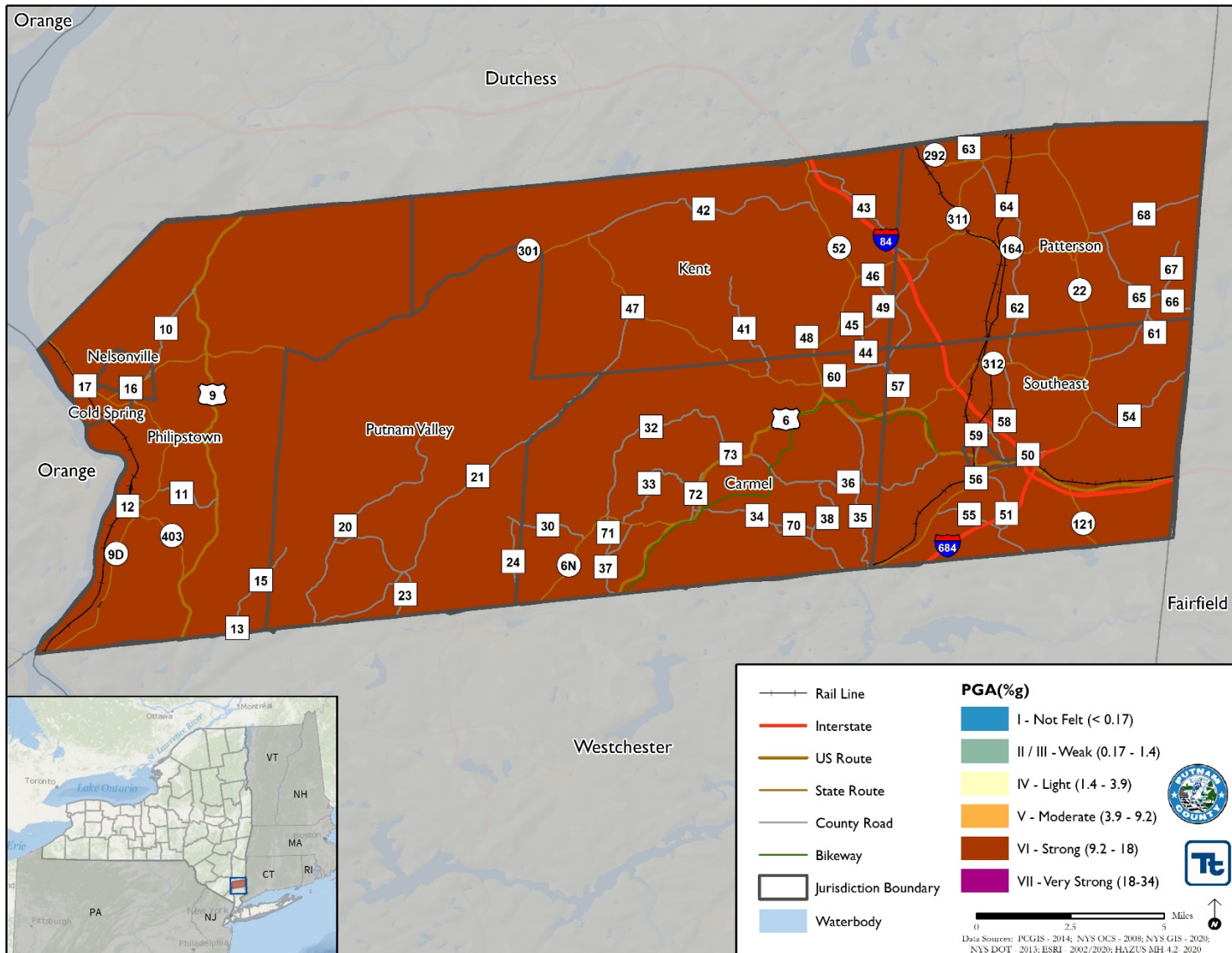
Figure 5.4.3-1. Peak Ground Acceleration Modified Mercalli Scale for a 2,500-Year MRP Earthquake Event
