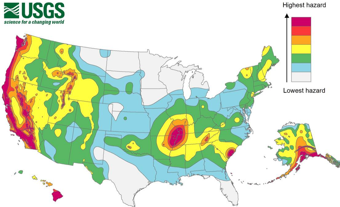
Figure 5.4.3-2. 2018 Long-Term National Seismic Hazard Map
