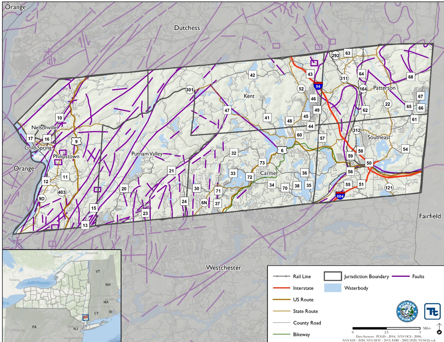
Figure 5.4.3-4. Fault Lines in Putnam County, New York
